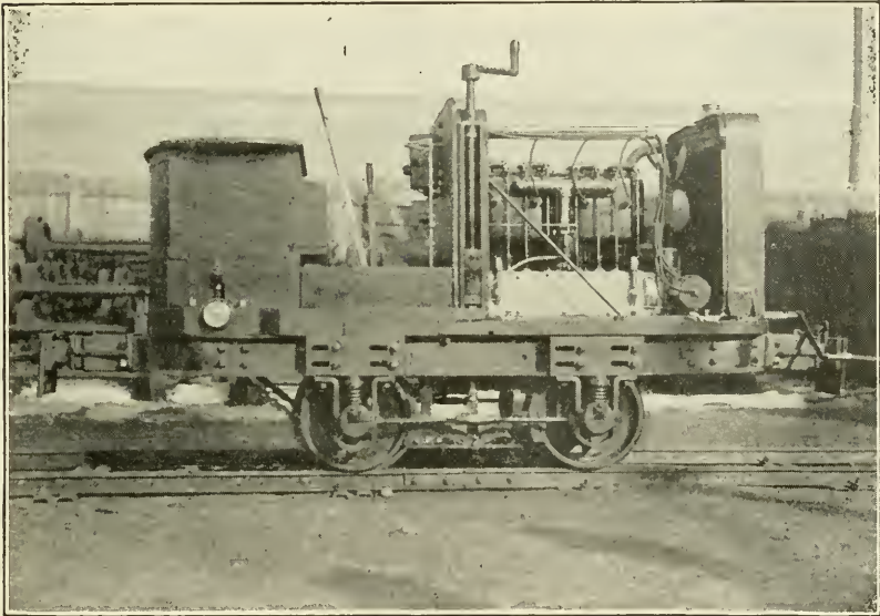
Fig. 5. Gasoline Industrial Locomotive.
